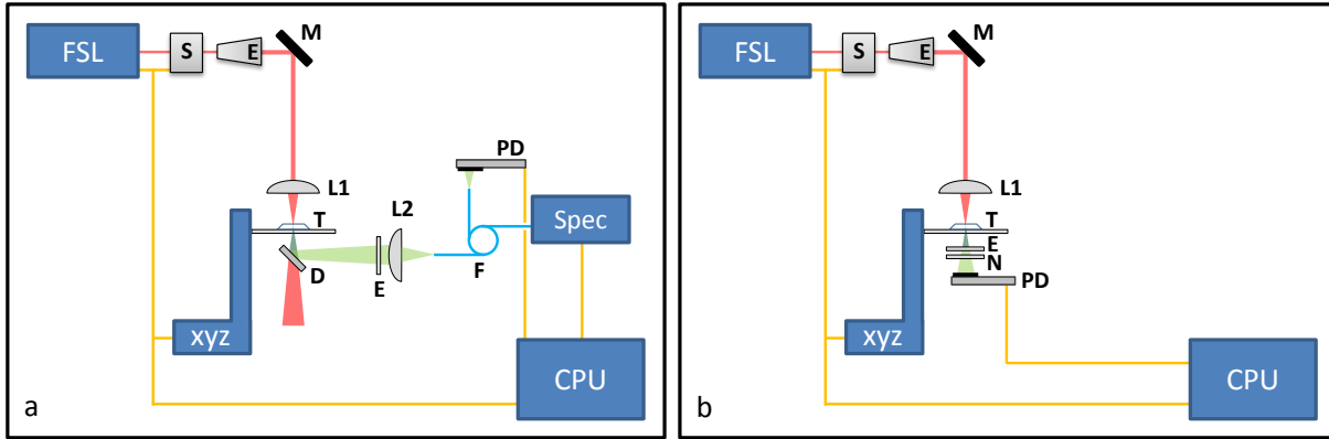
Figure 49. Principle optical experimental setup for measuring tissue (T) (a) second-harmonic generation intensity and duration of multiple pulses and (b) second-harmonic generation laser pulse energy and conversion efficiency of single pulses with respect to femtosecond laser (FSL) pulse energy using computer-controlled (CPU) translation stage (XYZ), laser and shutter (S). E beam expander; M mirror; L1, L2 lens; D dichroic beam splitter; SP short-pass filter; E edge-pass filter; N notch filter; PD photodiode sensor; F fiber; Spec spectrometer.
