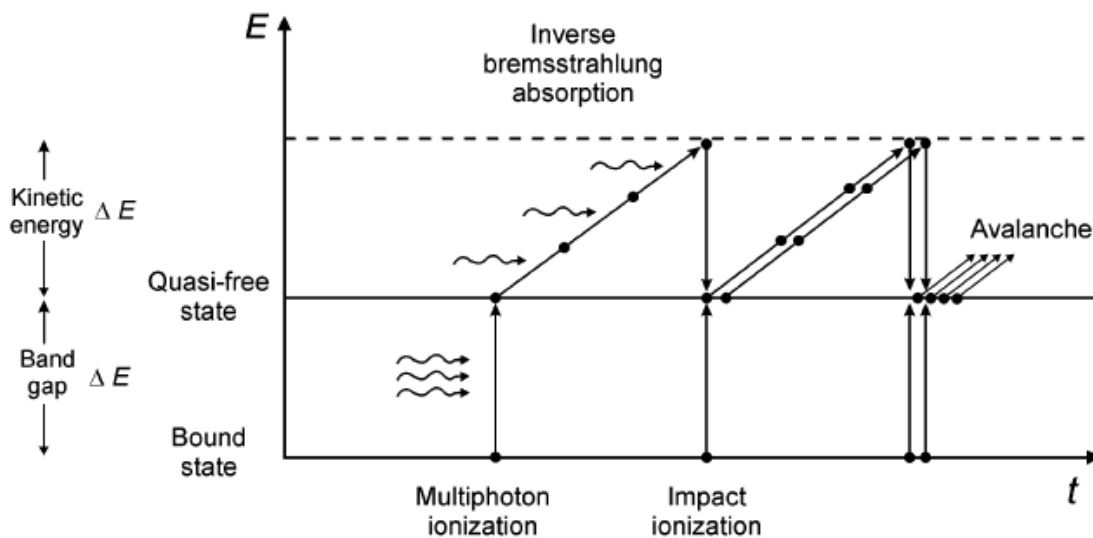
Figure 24. Description of avalanche ionization. Reprinted with permission from A. Vogel and V. Venugopalan, "Mechanisms of pulsed laser ablation of biological tissues," Chem Rev , vol. 103, pp. 577-644, Feb 2003. Copyright 2003, American Chemical Society.
